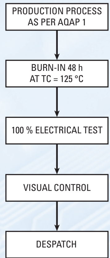
Process flowchart
