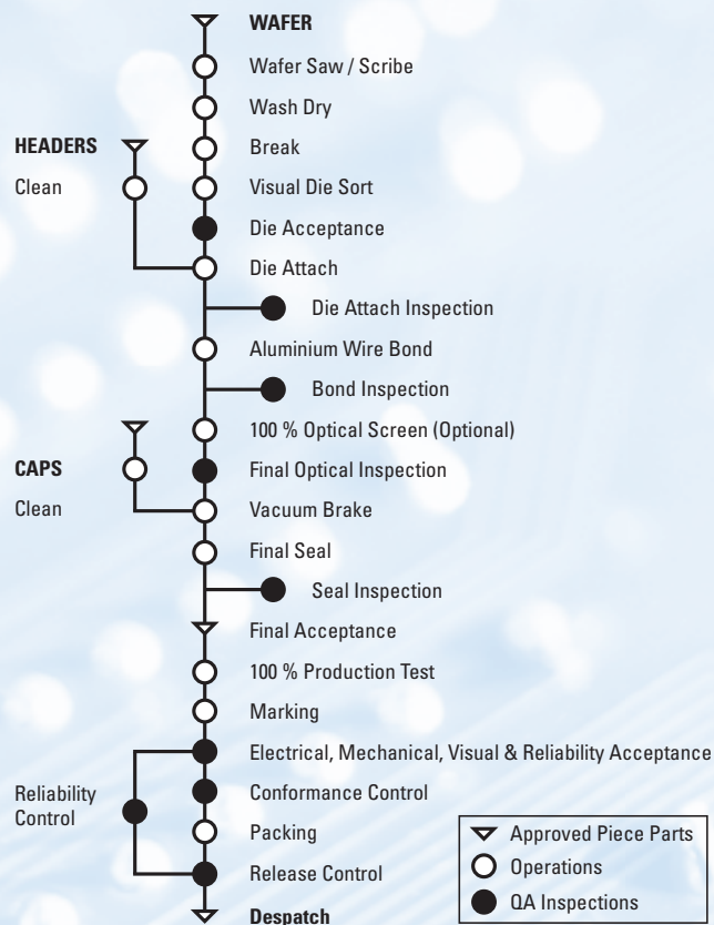
Manufacturing flowchart
